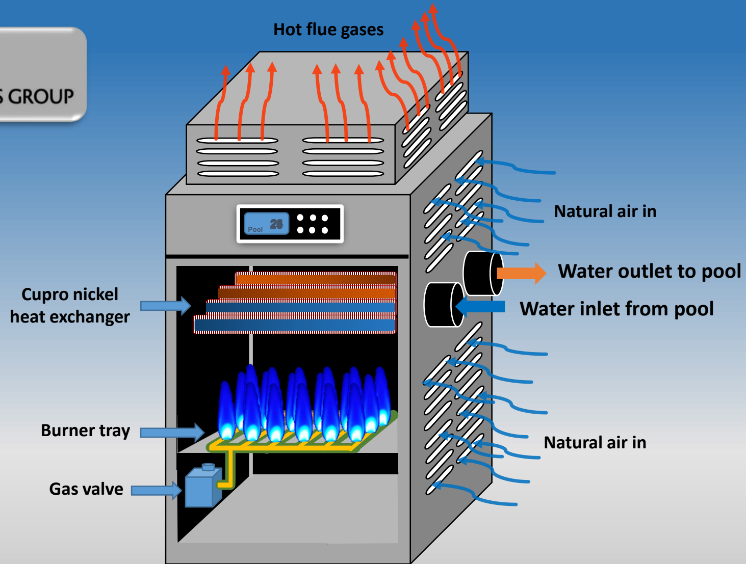
Representation of water heating process inside a Rheem gas pool heater
